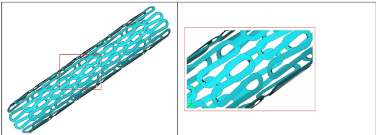
Figure 6. Structural integrity of the stent after the crimping process
