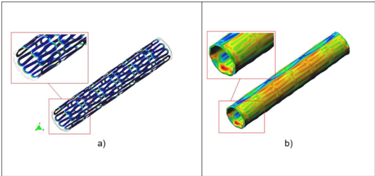
Figure 5. Principal deformation distribution (E1) of the stent and expandable balloon
