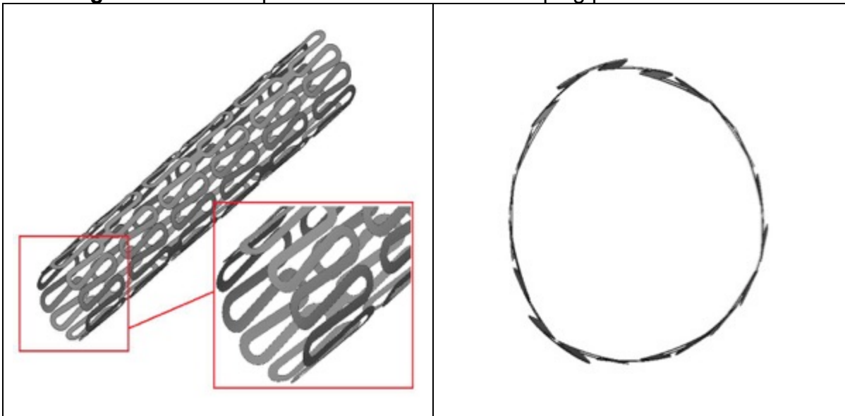
Figure 3. Final shape of the stent after the crimping process simulation
