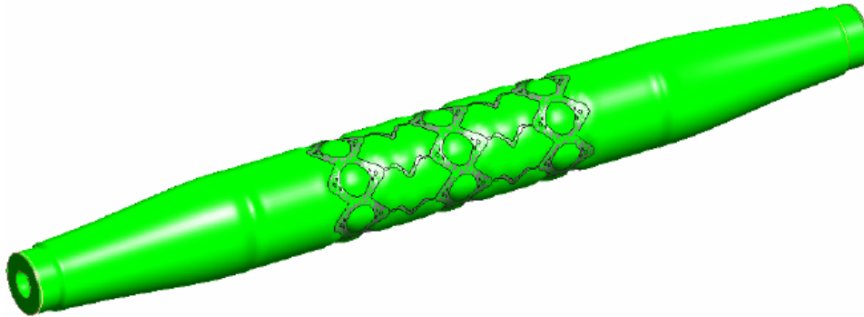
Figure 1. Simulation of the expansion of the stent and expandable balloon using finite elements (Langoni et al., 2006)
