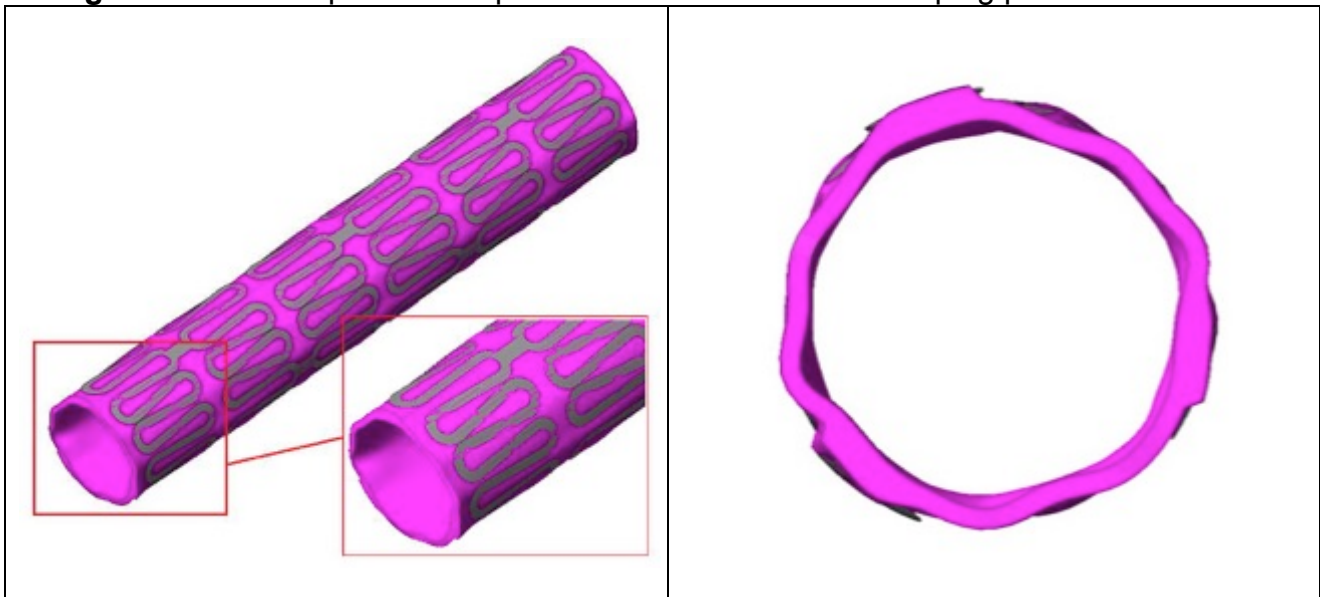
Figure 4. Final shape of the expandable balloon after the crimping process simulation
