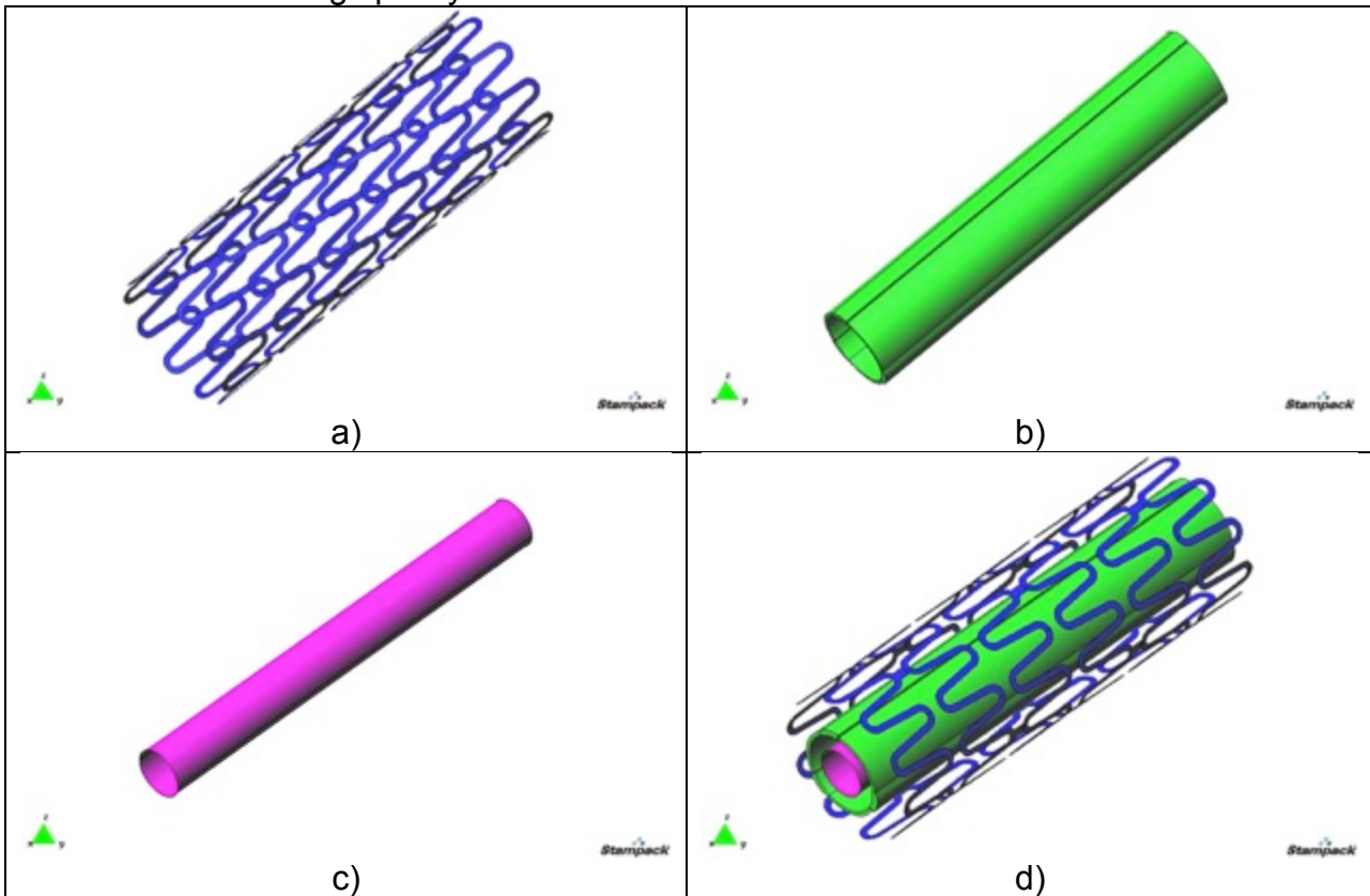
Figure 2. Geometrical models of the stent (a), expandable balloon (b), catheter (c) and (d) the set used in the angioplasty
